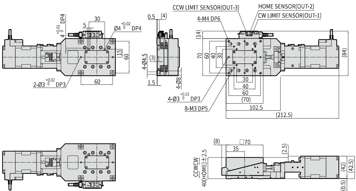
GNZ70-M TYPE
