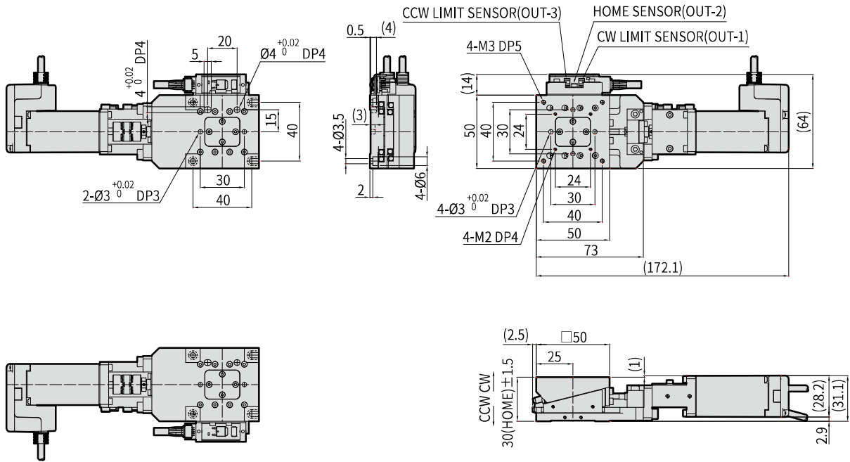
GNZ50-M TYPE
